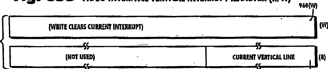
Fig. 35E VIDEO INTERFACE CURRENT LINE REGISTER
